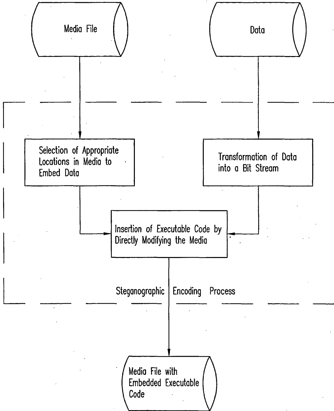
Data Encoding Using Steganographic Techniques
